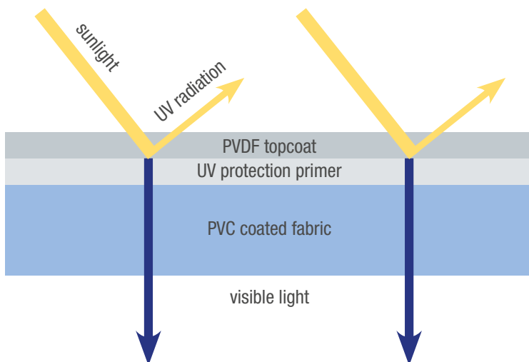
Protective effect of ROWAFLON® UV protection primers. The sensitive PVC surface is reliably protected against UV irradiation.
