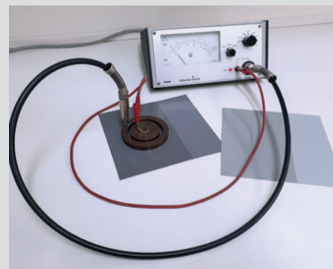
Measurement of surface resistance on PVC coated fabric using Teraohm meter and ring electrode. Left side lacquered with ROWAKRYL® G-34747W, right without lacquer.
